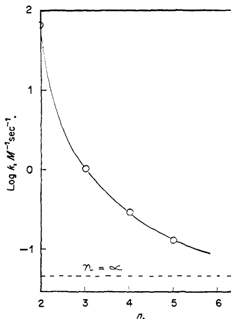
Figure 1. Dependence of the rate constant for the reaction of \text{Co}(\text{CN})_5^{3-} with \text{I}(\text{CH}_2)_n\text{I} on n . The dotted line designated n = \alpha denotes the rate constant for the reaction of \text{Co}(\text{CN})_5^{3-} with \text{CH}_3\text{CH}_2\text{CH}_2\text{I} .
